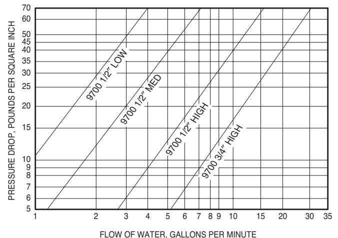
FLOW CAPACITIES SINGLE STAGE - SERIES 9700
