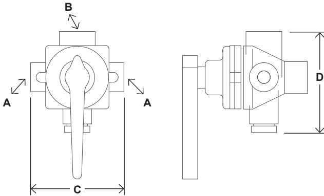
3000-SC1 with straight stop & check valves
